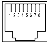
AUX2 connector (Model 55E rear panel)
