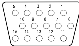
VGA/SVGA connector (Model 55E, rear panel)
