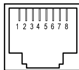
RJ45 connector (Model 55E rear panel)
